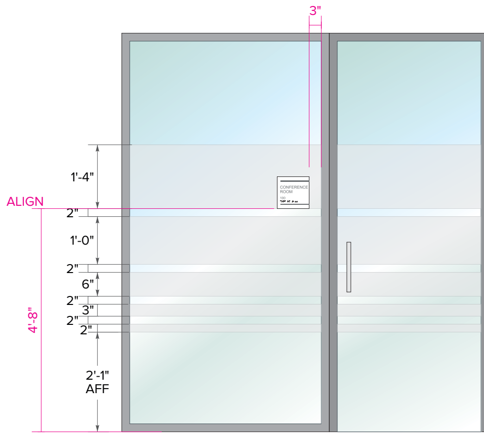
Typical Glass Sidelight Elevation
