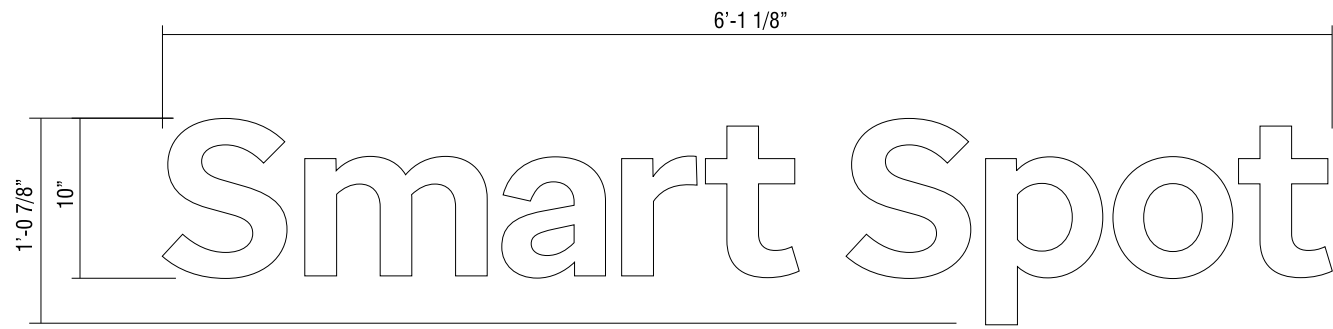
1a | 1 21 INTERIOR FCO LETTER LAYOUT - 10" SCALE: 1" = 1' 0"
