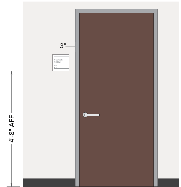
WALL MOUNT SCALE: 1/2" = 1'-0"
