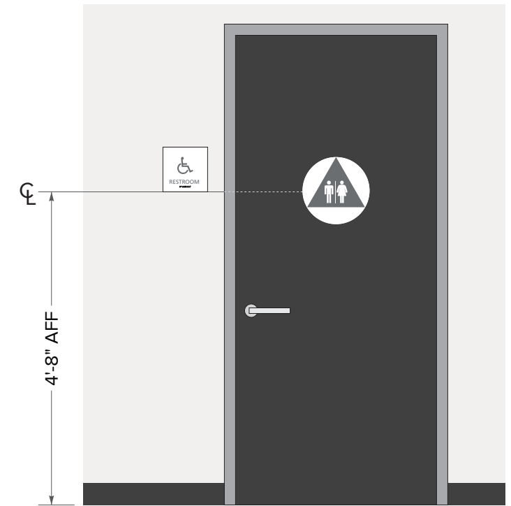
Typical Dark Colored Door Elevation
