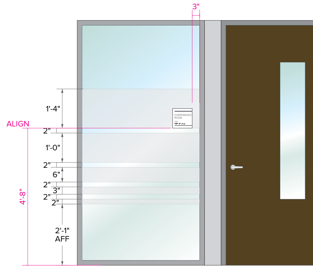
Typical Glass Sidelight Elevation
