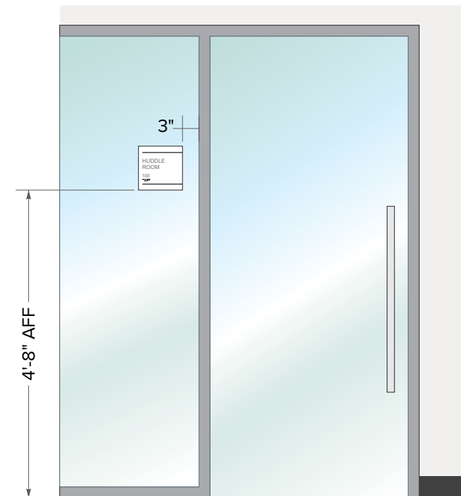
GLASS MOUNT - SIDE LIGHT SCALE: 1/2" = 1'-0"
