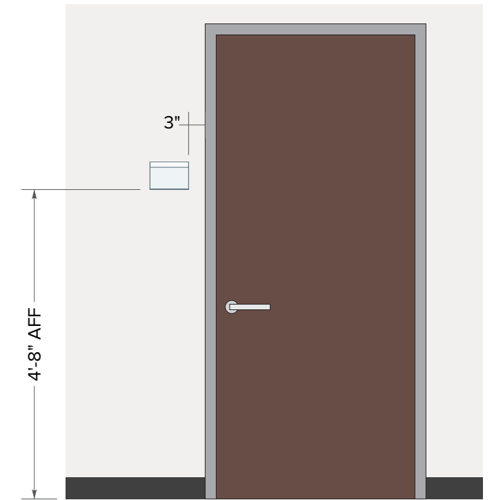
WALL MOUNT SCALE: 1/2" = 1'-0"
