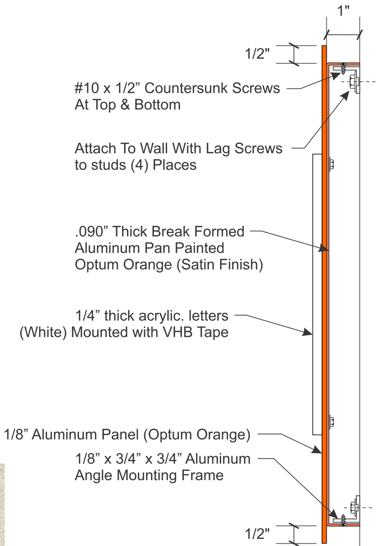
2 SECTION @ Reception Panel Sign SCALE: NTS
