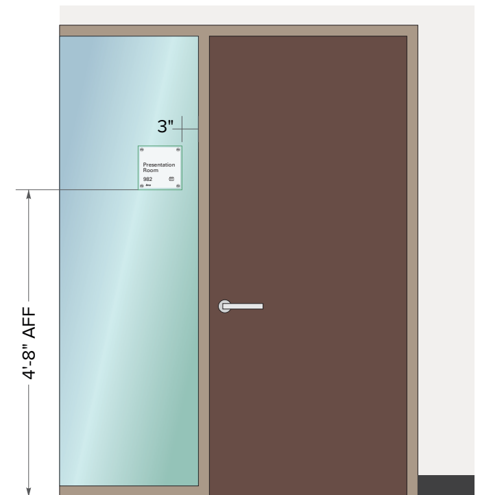
GLASS MOUNT SCALE: 1/2" = 1'-0"
