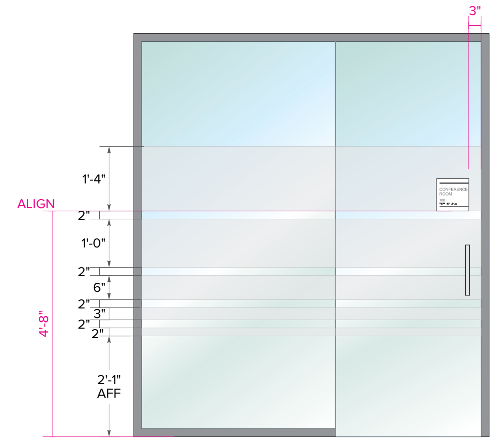
Typical Sliding Glass Door Elevation
